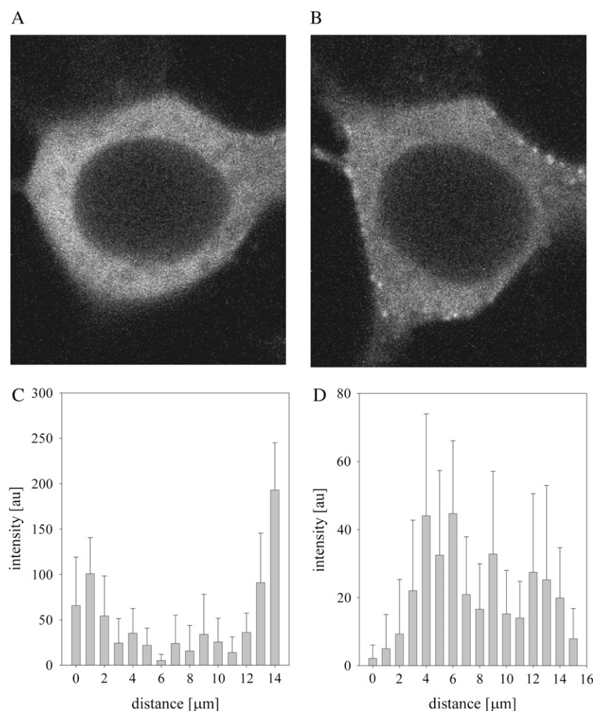
FIGURE 1 Image of a representative HEK293 cell expressing p85α/eYFP-p110α showing its cellular distribution after serum starvation for 24 h (A) and stimulation with 100 ng/mL of IGF-1 for 15 min (B). (C and D) Distribution of the eYFP-p110α intensity along a 3 × 3 pixel point along the z axis in a HEK293 cell and a C6 glial cell where the error is the standard deviation derived from the average of the nine pixels in the 3 × 3 sampling at each point (see Materials and Methods). The integration time is 6.4 μs/pixel.
