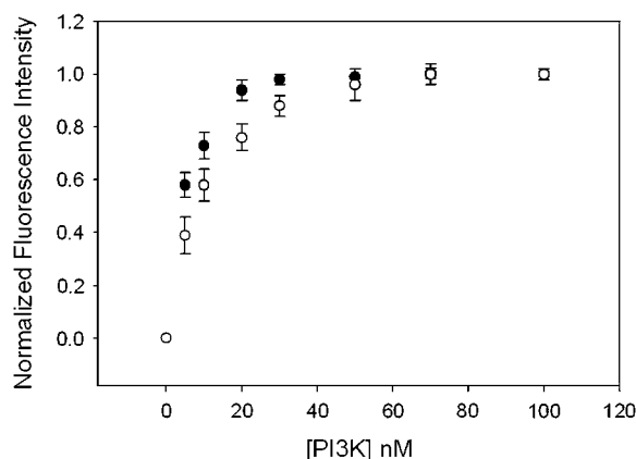
FIGURE 4 Binding of PI3K to 5 nM G\alpha_q (GTP \gamma S) in the absence and presence of PLC \beta . In vitro fluorescence binding assay showing the change in the normalized fluorescence intensity of 5 nM activated CM- G\alpha_q as purified PI3K is added, where the total increase in intensity was \sim 18\% . Experiments were performed in triplicate; the results are mean \pm SE.
